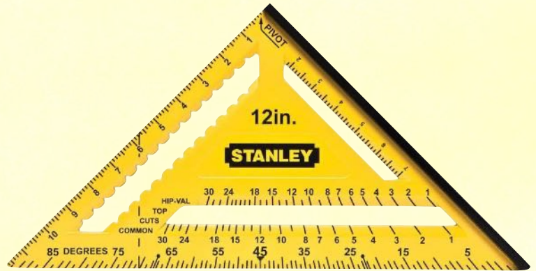
12" Dual Colour Quick Square SY046011
