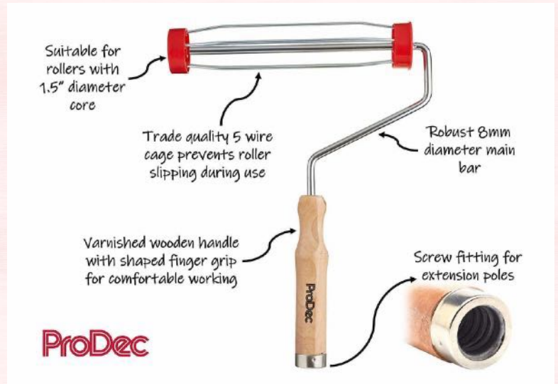
9" Wooden Handle Cage Frame RODO0040 / PRFR003
