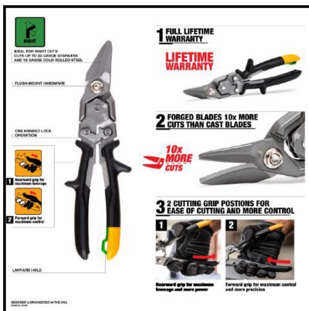
Right Aviation Snips TB020 / TH-H4-60-R
