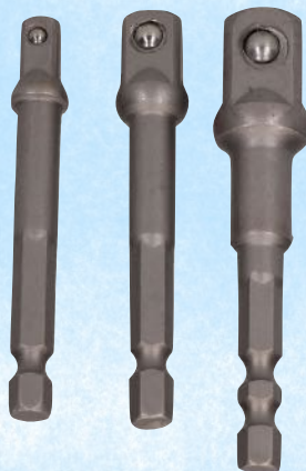
Power Extension 1/4"D, 3/8"D and 1/2"D LASER156 / 2981
